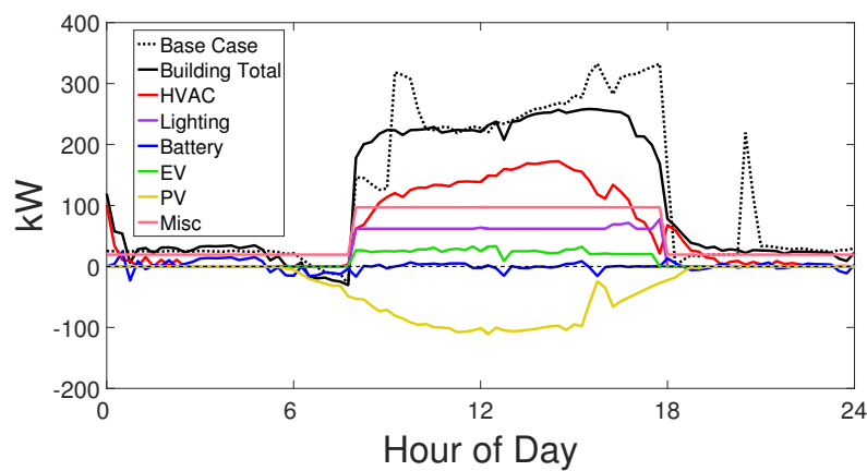
Figure 7. Power usage profiles for the whole building and for the individual subsystems during a “high solar” day under the Peak Demand model predictive control (MPC) with a five-hour horizon and perfect solar forecasting. The dashed profile represents the total building load under the rules-based control scheme.
