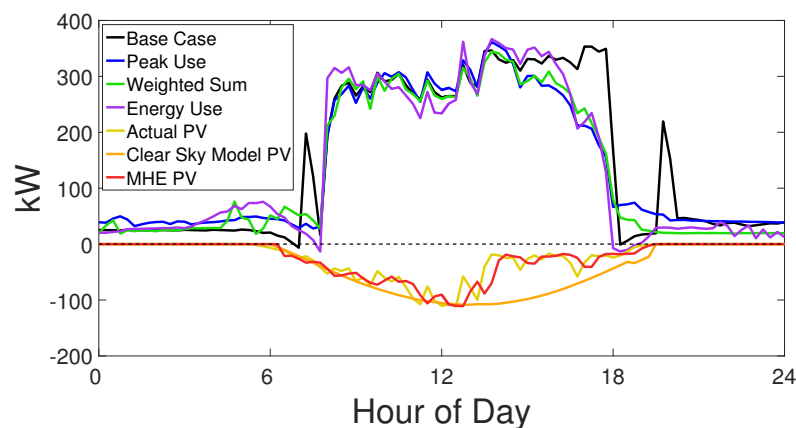
Figure 12. A comparison between the total building load profiles obtained under the rules-based control scheme (black line), the Peak Demand MPC (blue line), the Net Energy Use MPC (purple line), the Weighted Sum MPC (green line), all with a fifteen-minute moving horizon solar forecast and a five-hour MPC horizon for the “low solar” day. The actual solar power availability is shown by the yellow profile; the clear sky model’s predicted solar power by the orange profile, and the estimated solar availability based on the moving horizon estimation scheme by the red profile.
