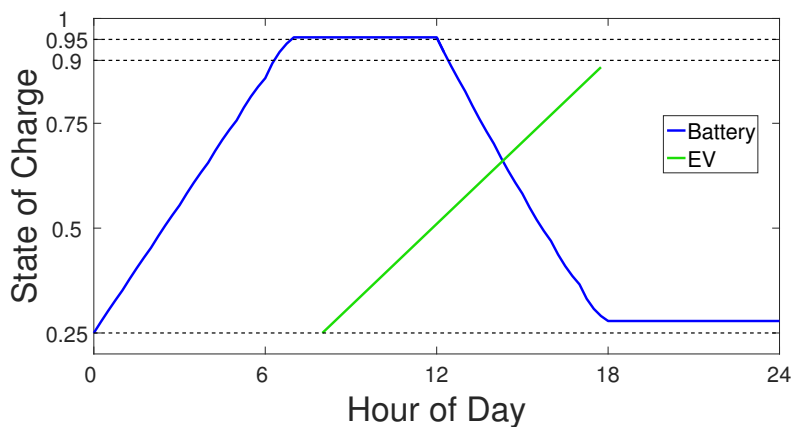
Figure 4. State of charge for the battery storage and electric vehicle (EV) system under the rules-based base case.
