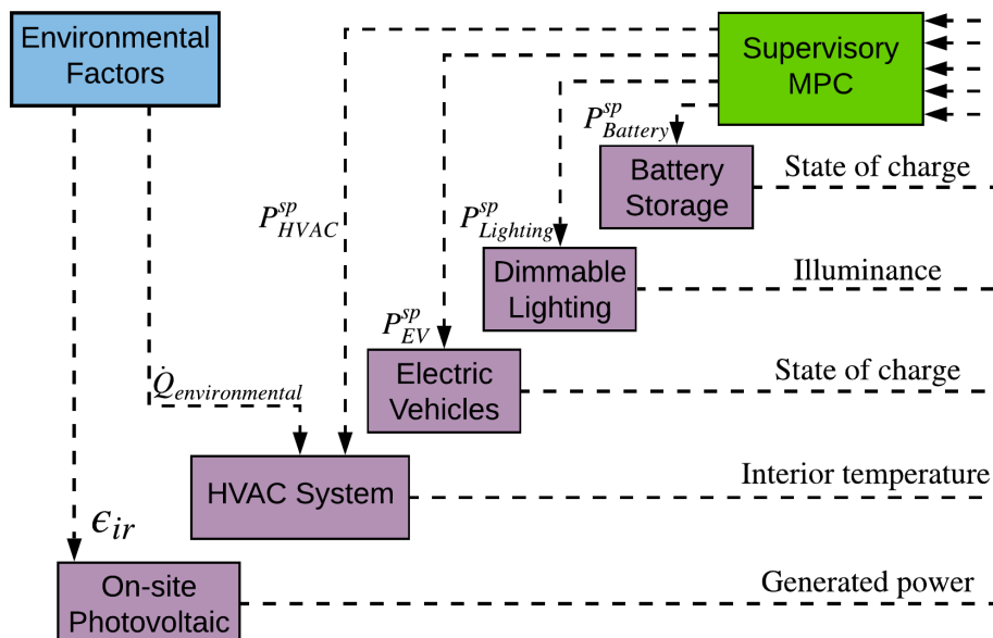
Figure 1. Supervisory control, optimization and coordination structure.
