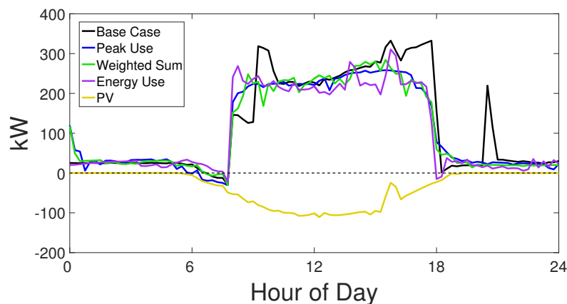
Figure 10. A comparison between the total building load profiles obtained under the rules-based control scheme (black line), the Peak Demand MPC (blue line), the Net Energy Use MPC (purple line), the Weighted Sum MPC (green line), all with perfect solar forecasting and a horizon length of 5 hours, for the “high solar” day. The solar power generation profile is indicated by the yellow line.
