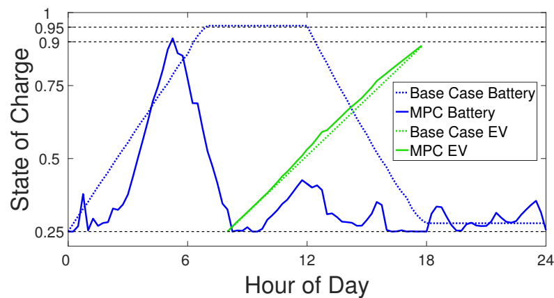
Figure 9. Typical state of charge for the battery storage and EV subsystems under the supervisory MPC system, referenced with the state of charge for the same subsystems in the rules-based base case.
