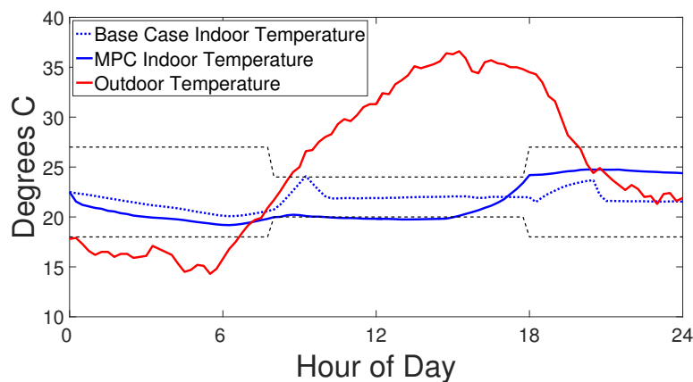
Figure 8. Indoor building temperature profiles under the rules-based control scheme and under the supervisory Peak Demand MPC with perfect forecasting, with upper and lower indoor temperature bounds (dashed black line), referenced with the ambient outdoor temperature.
