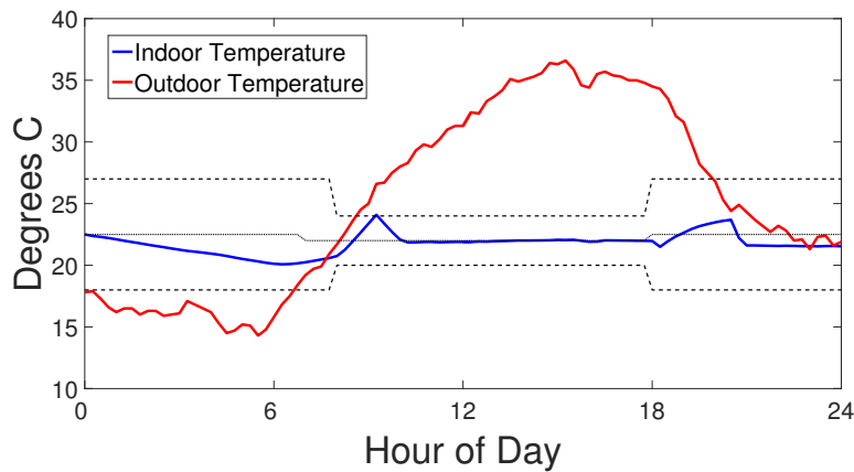
Figure 3. Time profiles of the building's indoor and outdoor temperatures under the rules-based control scheme.
