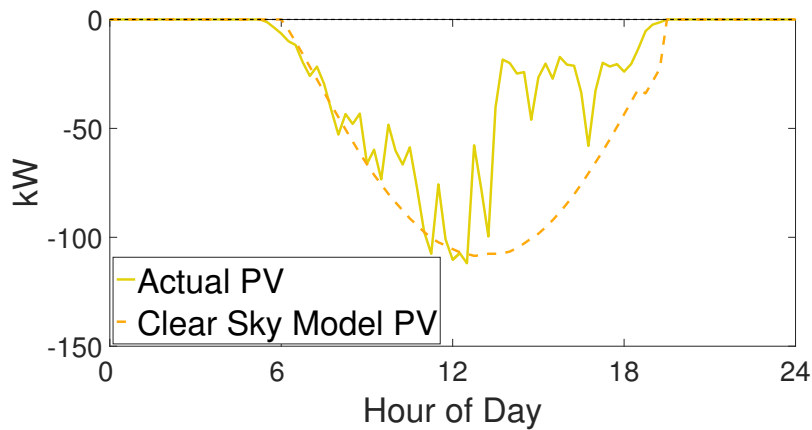
Figure 6. A comparison between actual PV power availability (solid line) and the power predicted by the clear sky model (dashed line) for a simulated day with low solar irradiance (1 July 2015).
