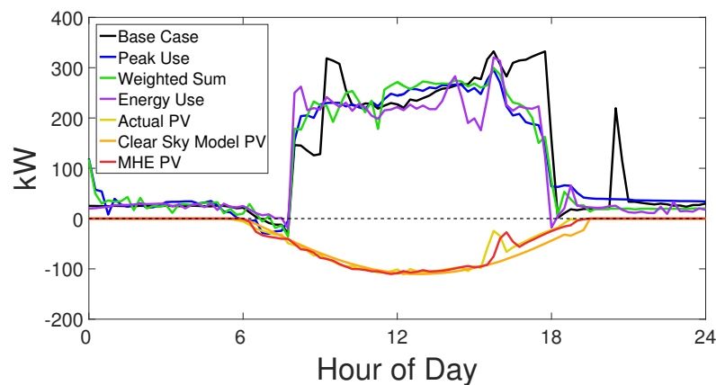
Figure 11. A comparison between the total building load profiles obtained under the rules-based control scheme (black line), the Peak Demand MPC (blue line), the Net Energy Use MPC (purple line), the Weighted Sum MPC (green line), all with a fifteen-minute moving horizon solar forecast and a five-hour MPC horizon for the “high solar” day. The actual solar power availability is shown by the yellow profile; the clear sky model predicted solar power by the orange profile, and the estimated solar availability based on the moving horizon estimation scheme by the red profile.
