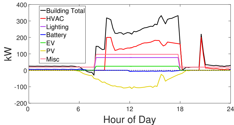
Figure 2. Power consumption profiles for the building and the individual subsystems under rules-based control scheme over a 24 h period.
