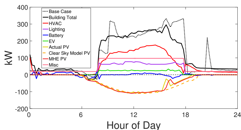
Figure 13. Power usage profiles for the entire building and the individual subsystem under the Peak Demand MPC with a fifteen-minute moving horizon solar forecast and a five-hour MPC horizon, referenced with the total building load under the rules-based control scheme.
