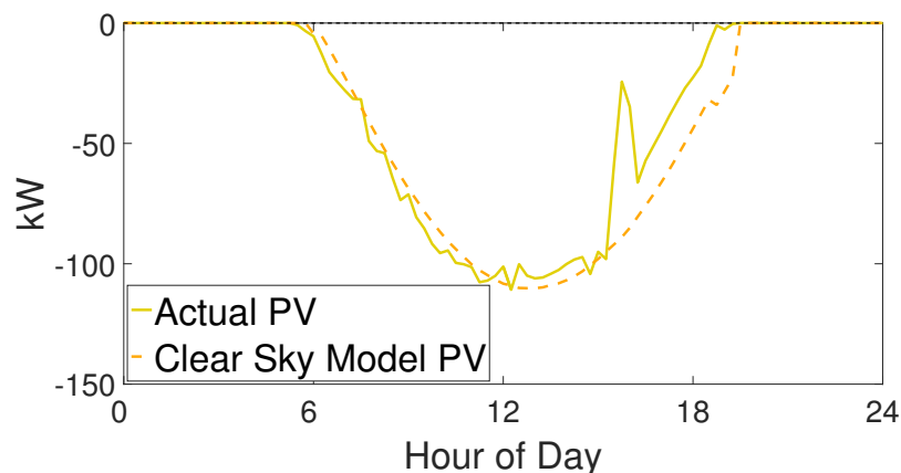
Figure 5. A comparison between actual photovoltaic (PV) power availability (solid line) and the power predicted by the clear sky model (dashed line) for a simulated day with high solar irradiance (29 June 2015).
